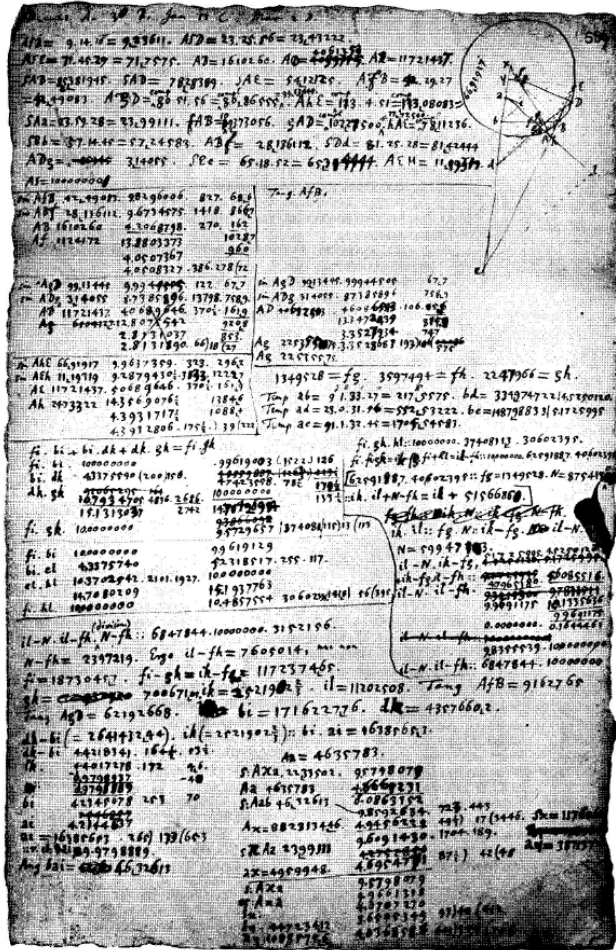
Newton
